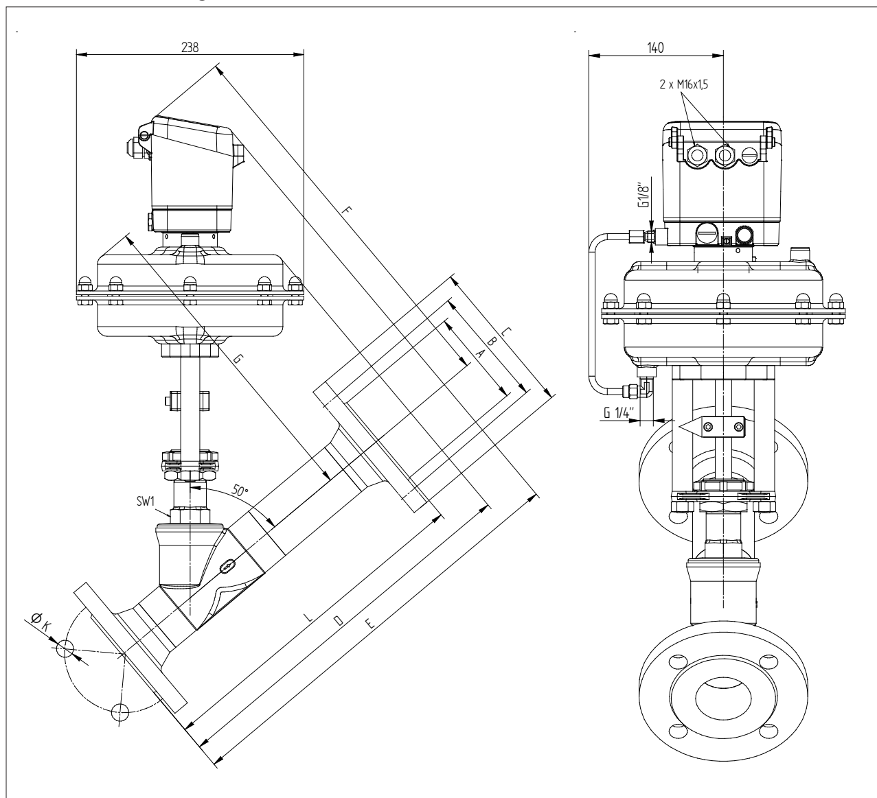
diaphragm actuator with digital positioner 8049
