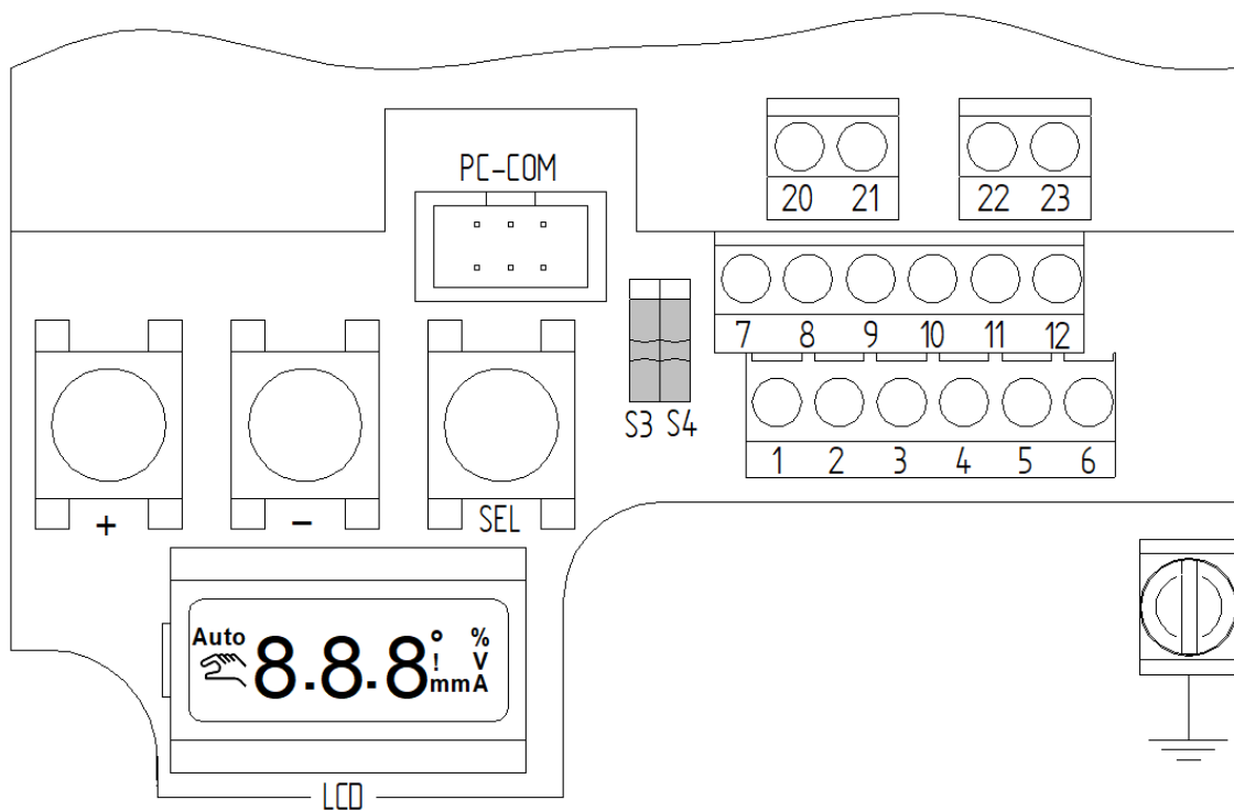
Terminal assignment 24V-Version
